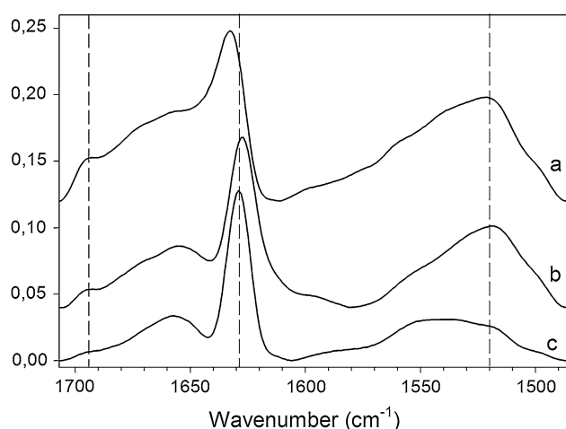
Fig. 4 ATR-FTIR spectra of A \beta (1–40) in the amide I and II regions. A \beta (1–40) in TBS, pH 7.4, a after 0 h, b after 24 h, and c after 96 h. Spectral intensities were normalized to the intensity of the 1,630 \text{cm}^{-1} peaks and were shifted for better visualization. Spectra were deconvoluted using a Lorentzian deconvolution factor with a full width at half height of 20 \text{cm}^{-1} and a Gaussian apodization factor with a full width at half height of 13.33 \text{cm}^{-1} to obtain a resolution enhancement factor K = 1.5 . Spectra are representative of at least three independent experiments
